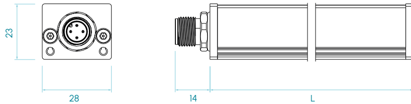
Motion sensor + M12A axial input
