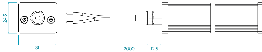
Motion sensor + M12A axial input
