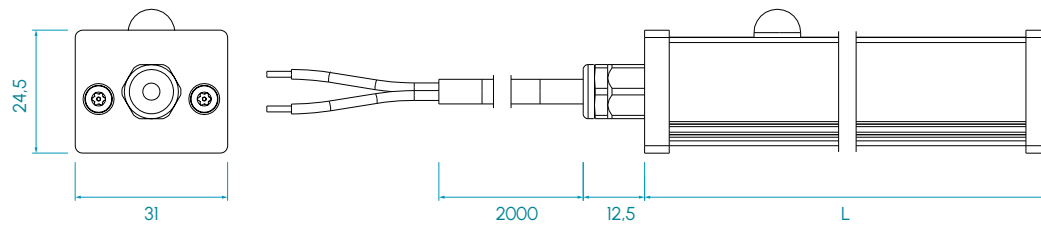
Motion sensor + M12A axial input
